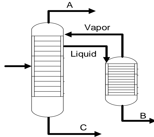
SIDE STREAM STRIPPER
